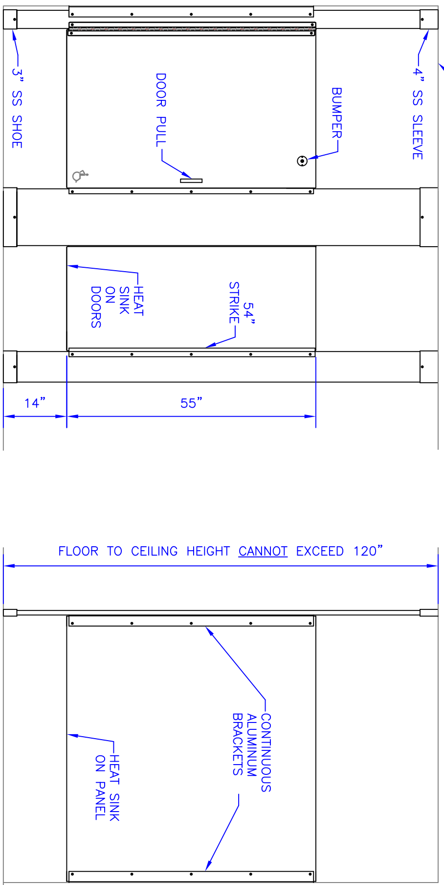
FRONT ELEVATION
